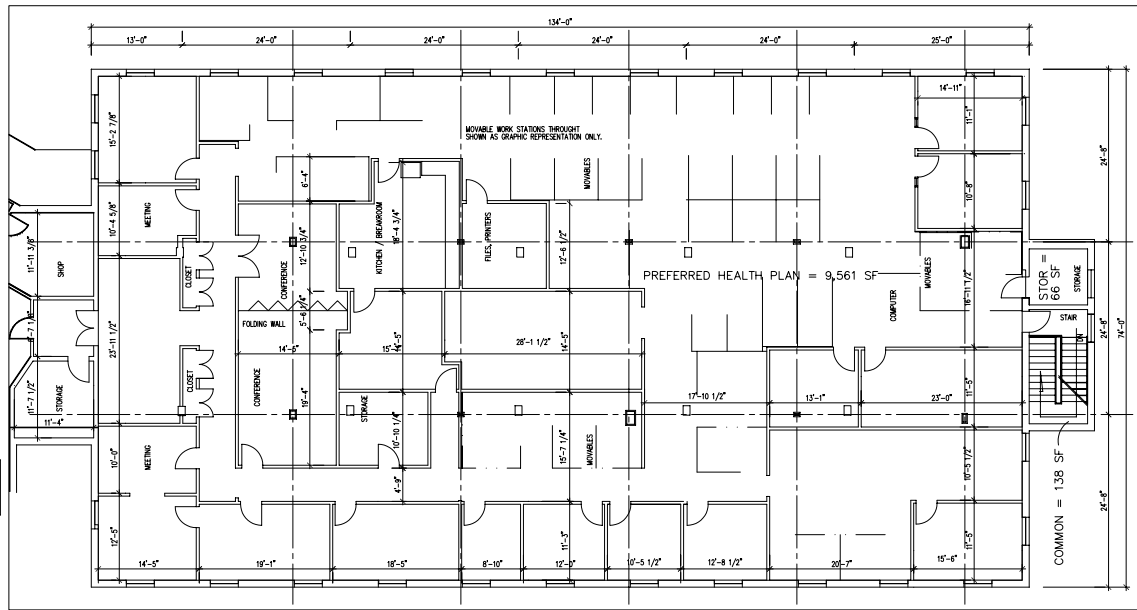
WING "B" SECOND FLOOR PLAN SCALE: 1/8"=1'-0"
