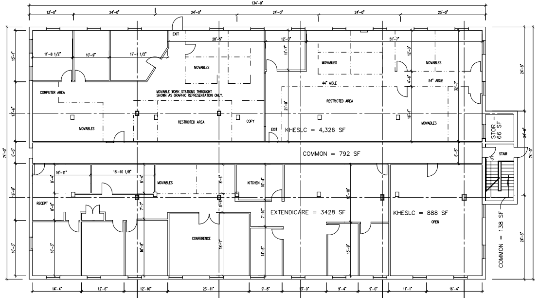
WING "B" FIRST FLOOR PLAN SCALE: 1/8"=1'-0"
